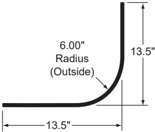
6" RADIUS PANEL
