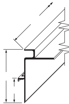
NOSE RAIL, 93"
