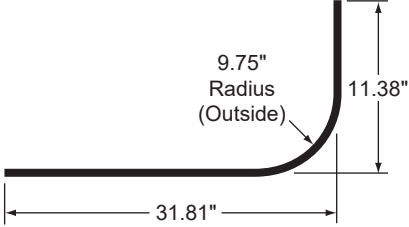
10" RADIUS PANEL Stoughton Number DOR-FB30382
