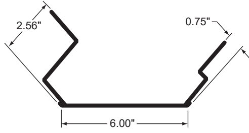
CORNER POST, 110.31", MILL
