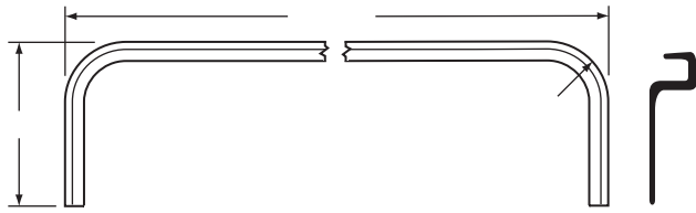
NOSE RAIL, ALUM
