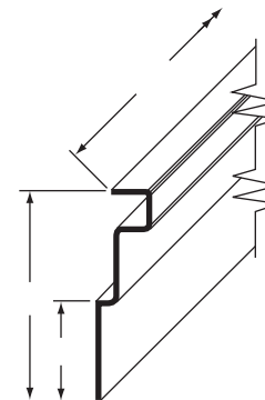
NOSE RAIL, 91.25"
