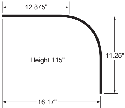
RADIUS PANEL, TM RP102K-PPW
