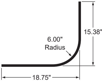
6" RADIUS PANEL, SS
