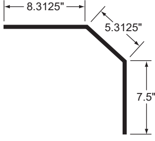
RADIUS PANEL, BEVEL, FRONT Stoughton Number DOR-FR2804118
