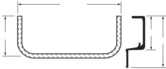
6" NOSE RAIL, ALUM, 102-3/8"
