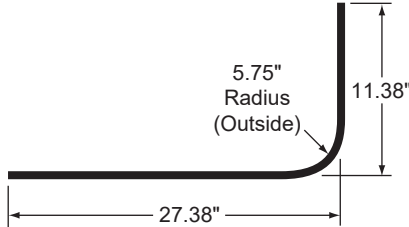
5.7" RADIUS PANEL, PPW Stoughton Number DOR-FA30783
