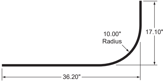
10" RADIUS PANEL, PPW
