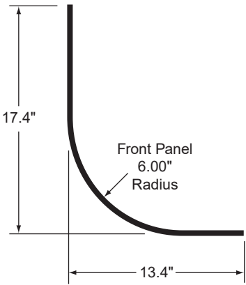
6" RADIUS PANEL W/ PVC
