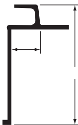
5" TRAILER HEADER, PLATE, 102"
