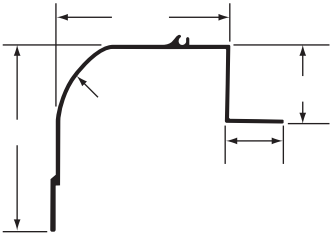
CORNER POST, ALUM, 112.5"
