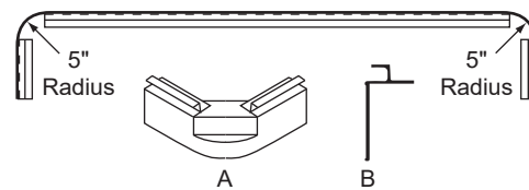
5" TRAILER HEADER, PLATE, 102"
