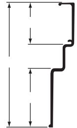
TOP RAIL, FRONT, ALUM, 101-7/8"
