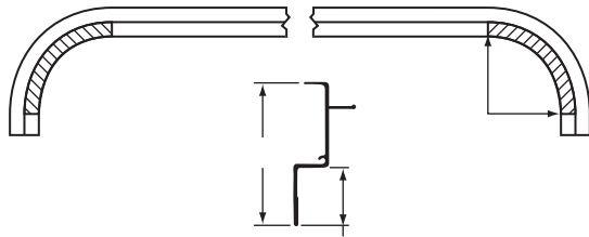
NOSE RAIL, 102" Stoughton Number WAB-04A00005
