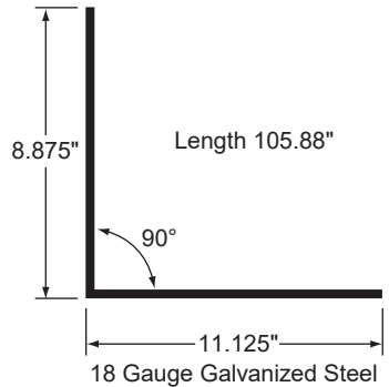
CORNER POST LINER, GALV, 105.88"
