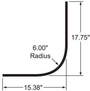
CORNER RADIUS, PPG
