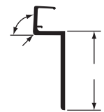
TOP RAIL, FRONT, ALUM, 101-7/8"
