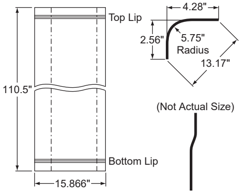
6" RADIUS PANEL, SST
