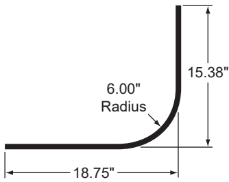
6" RADIUS PANEL, CS 100-1/4"
