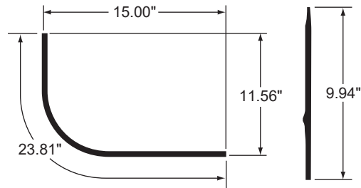
CORNER RAIL, LOWER LEFT HAND
