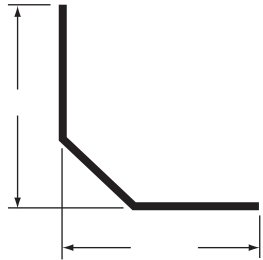
RADIUS PANEL, WHT, ALUM
