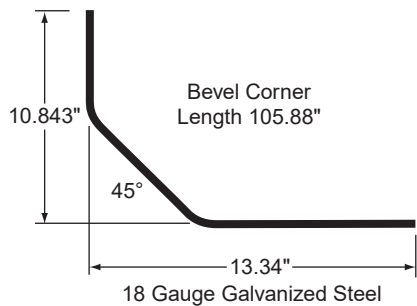
CORNER POST LINER, WHT, GALV
