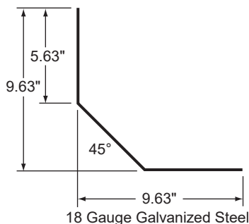
CORNER LINER, G90 GALV, MILL
