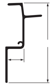
5" NOSE RAIL, ALUM, 102" Stoughton Number WAB-04A02464
