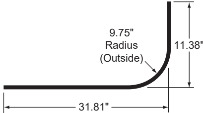
10" RADIUS PANEL Stoughton Number DOR-FR30382
