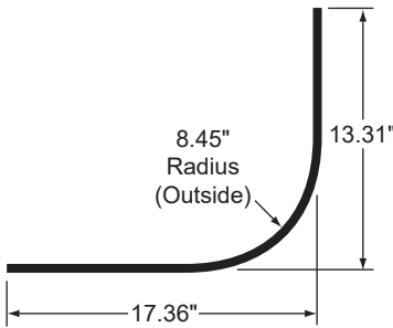
8.45" RADIUS PANEL, WHT, ALUM
