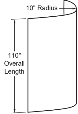
10" RADIUS PANEL, MILL FINISH Stoughton Number FRU#WCC8051-SPN
