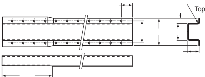
NOSE POST, STEEL, UNPUNCHED, 116"
