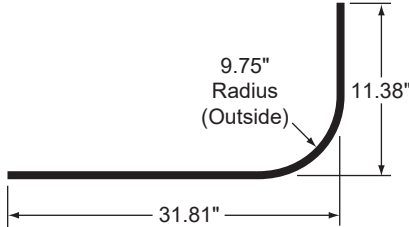
10" RADIUS PANEL, PPW Stoughton Number DOR-FA30382
