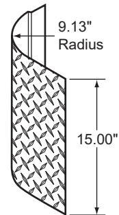
9.125" CORNER PROTECTOR
