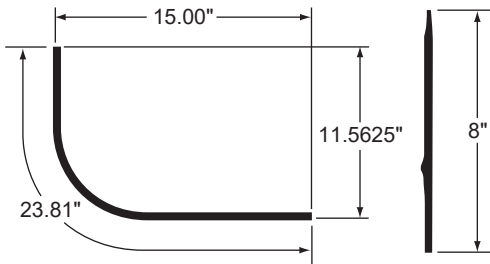
CORNER RAIL, LOWER LEFT HAND
