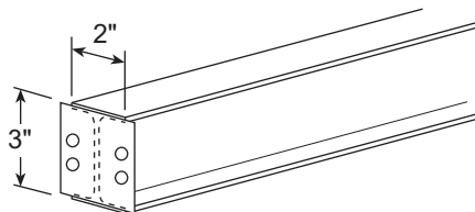
3" CROSSMEMBER ASSEMBLY
