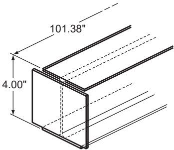
CROSSMEMBER, 4" x 101.38"
