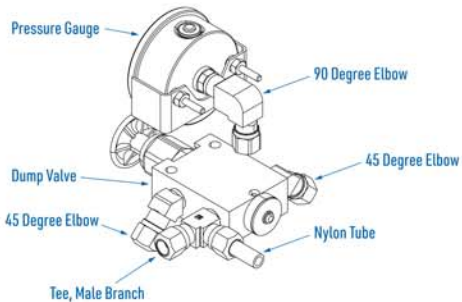
DUMP VALVE
