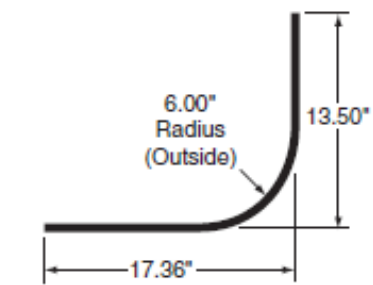
6" RADIUS PANEL, PPW W/PVC 11
